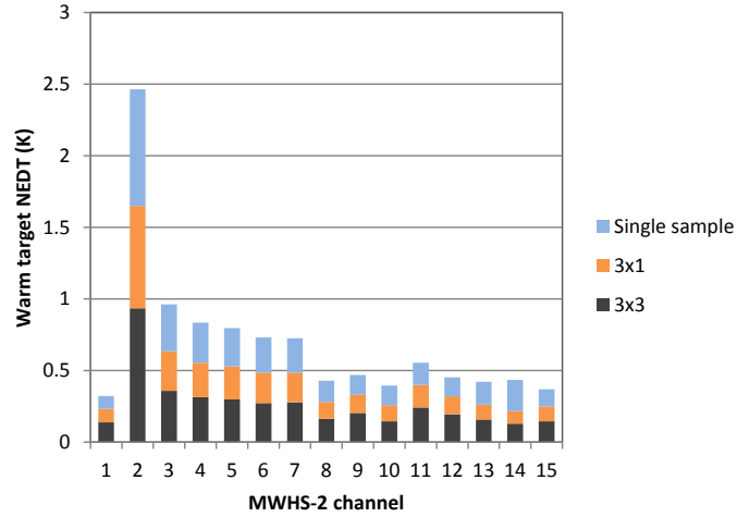
Figure 20: NE\Delta T for MWHS-2, similar to Fig. 11.
